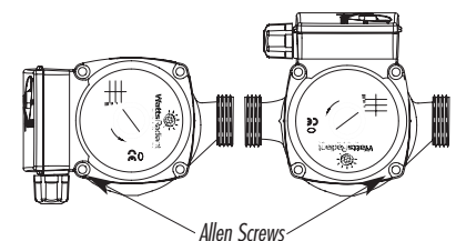
Remove allen screws to rotate pump head. Should only be done if necessary to fit an enclosure.
